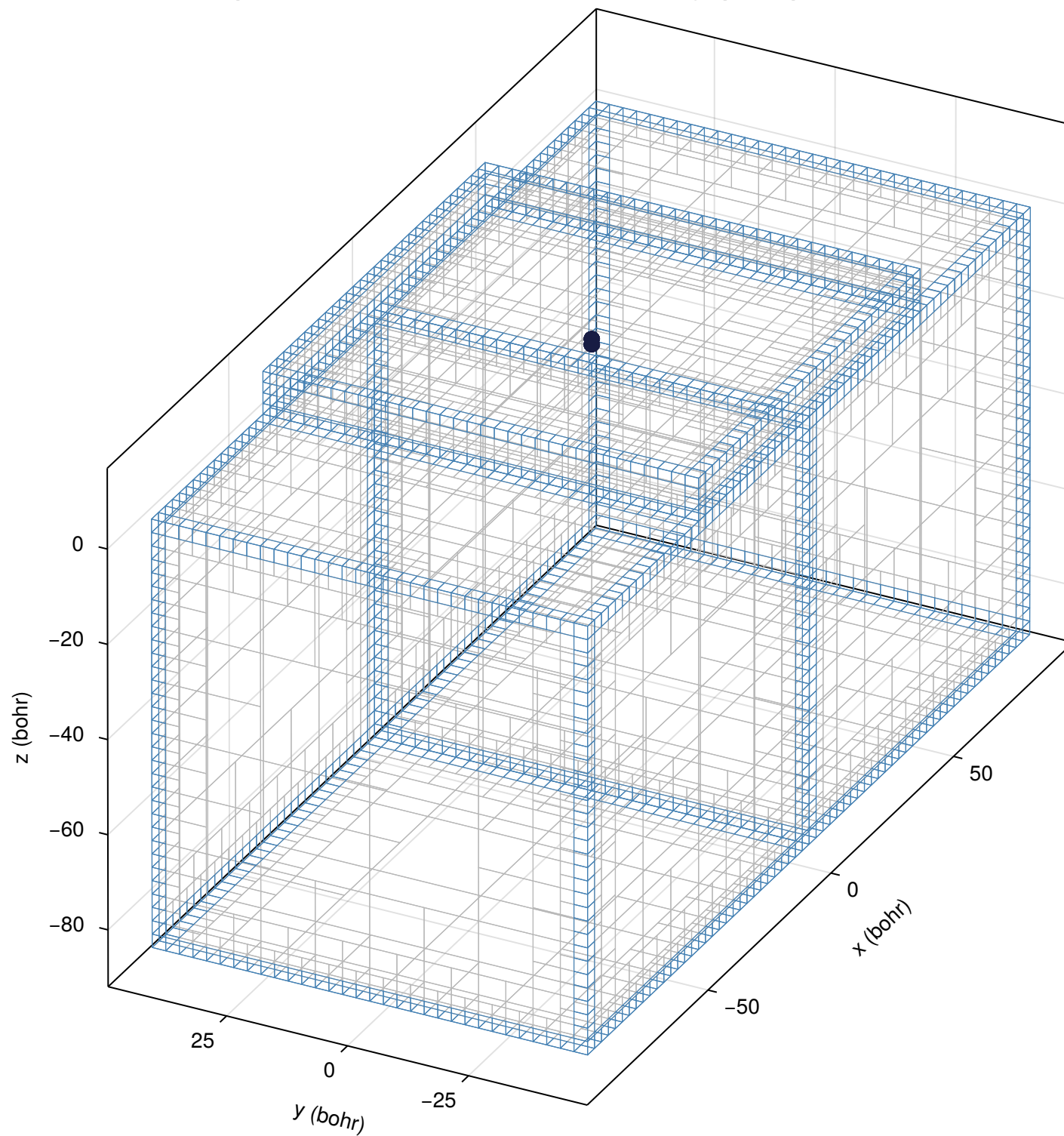
exp66: two 90^3 cubes ( \epsilon 11.9 | 3.9) + slab ( \epsilon 10), graphene p_z orbital source
