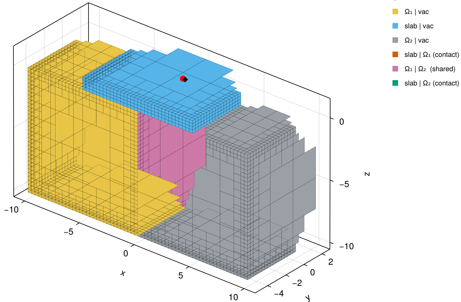
Fig.-1 system: 10 \times 10 \times 1 slab ( \epsilon=10 ) on two 10 \times 10 \times 10 cubes ( \epsilon=4, \epsilon=12 )
