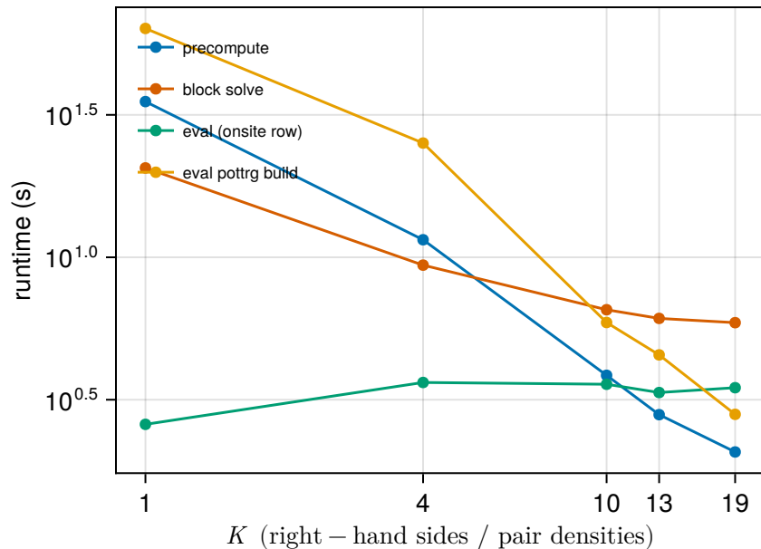
(a) runtime vs K
