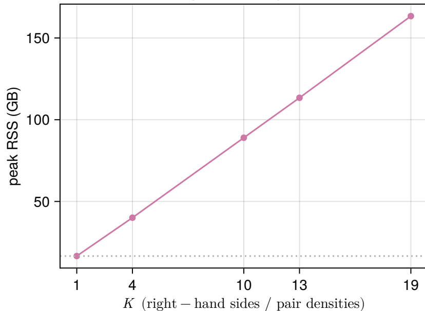
(b) peak memory vs K
