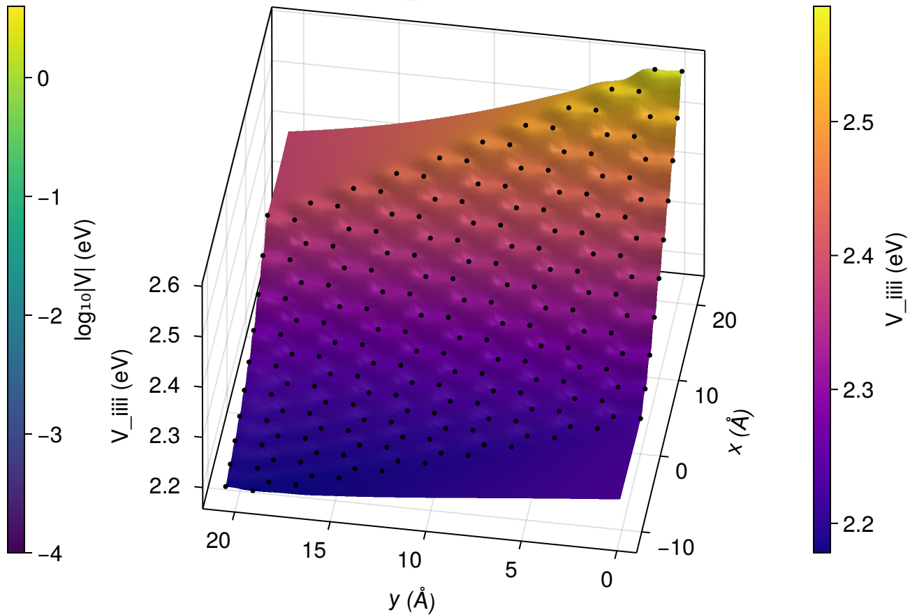
onsite U_i over the lattice
