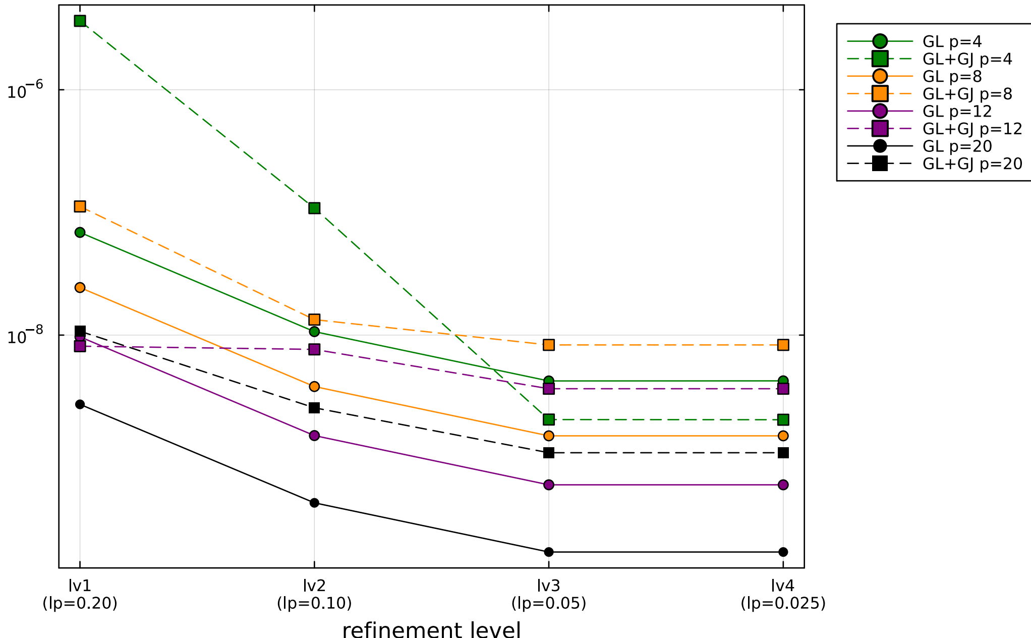
h-convergence at fixed p ( \varepsilon_{\text{in}}=1 , \varepsilon_{\text{out}}=200 )
