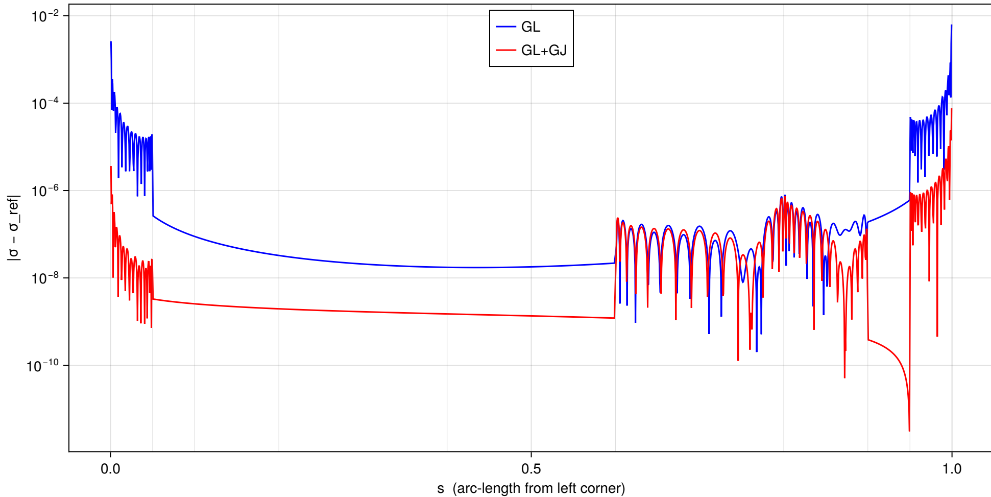
Density error along full edge n=16 , lc=0.05 , \epsilon_{in}=1.0 , \epsilon_{out}=200.0
