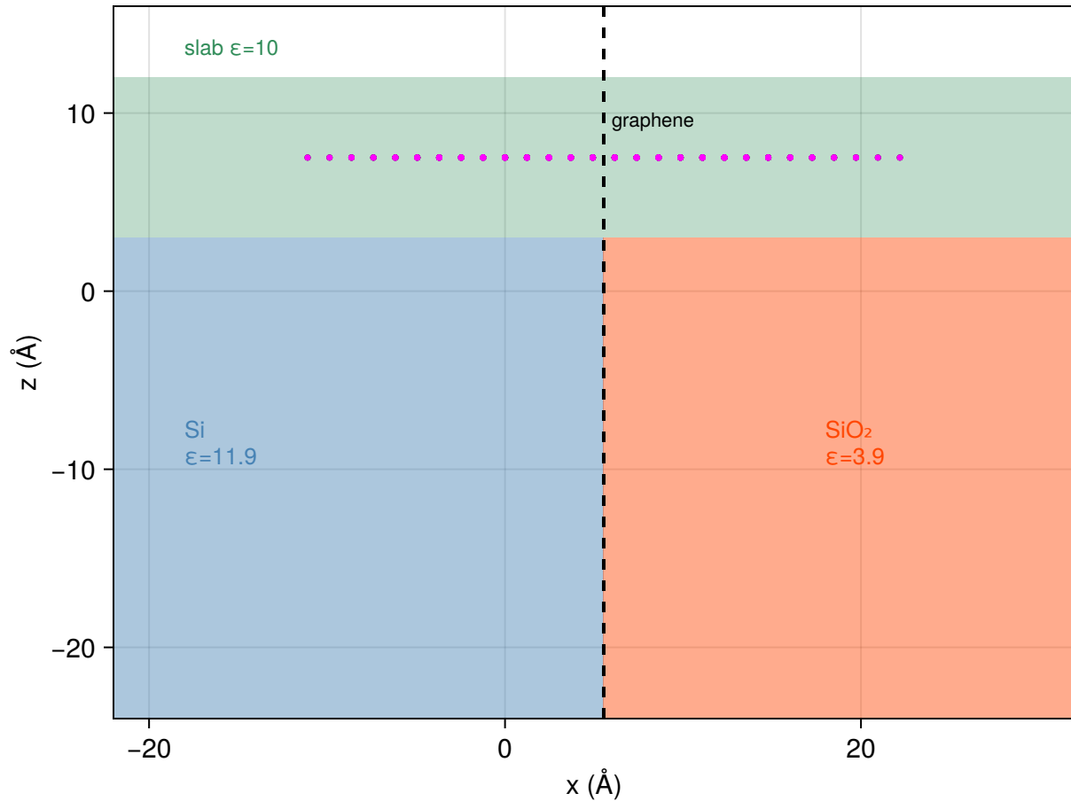
side view (x-z): Si | SiO 2 substrate + slab
