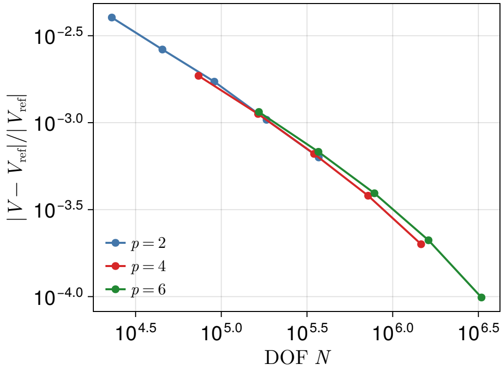
(a) convergence, slab on two cubes (Fig. 1), \varepsilon = 10^{-4}
