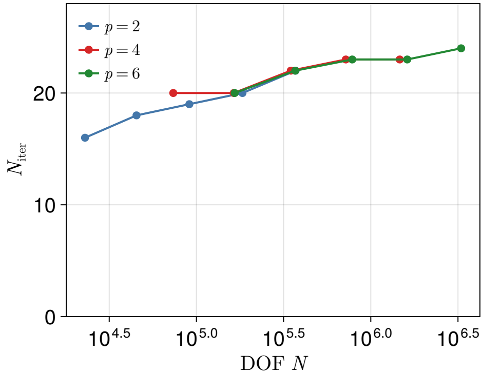
(b) GMRES iterations
