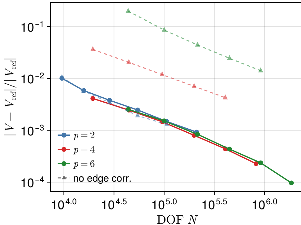
(a) convergence, slab 10 \times 10 \times 1 , \epsilon = 10^{-4}
