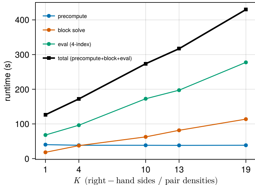
(a) runtime vs K (96 threads, FINUFFT→16 in-function)
