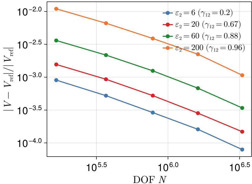
(a) convergence vs contrast ( p = 6 ), \varepsilon = 10^{-4}
