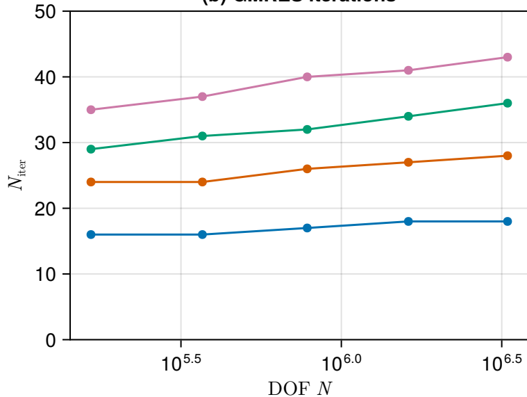
(b) GMRES iterations
