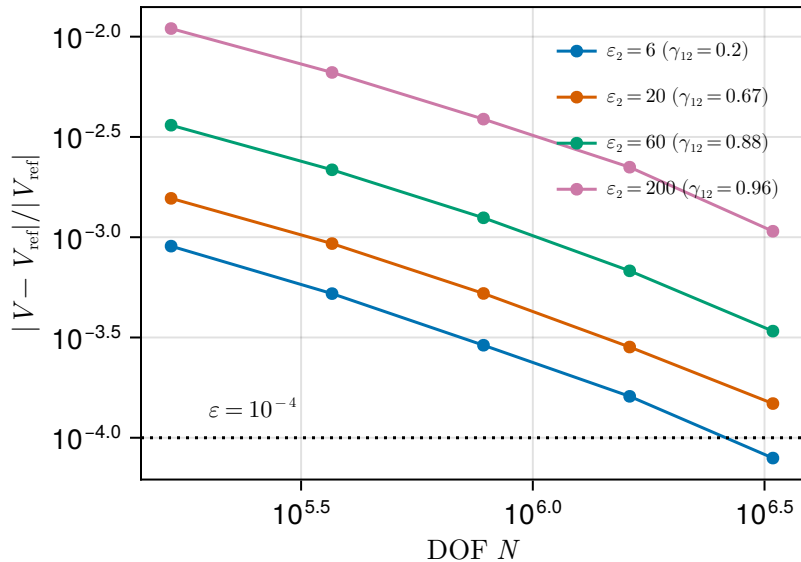
(a) convergence vs contrast ( p = 6 ), \varepsilon = 10^{-4}
