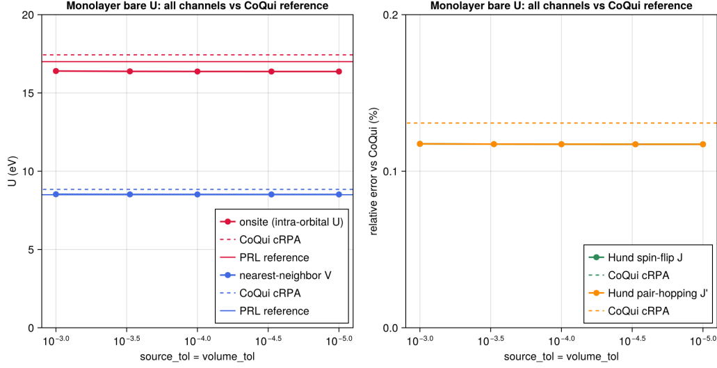
FIG. 1: All four bare channels (onsite, NN, Hund's spin-flip, Hund's pair-hopping) versus quadrature tolerance. Dots are this work; dashed horizontal lines are the CoQui cRPA bare references; and solid lines are the PRL 106, 236805 values.
