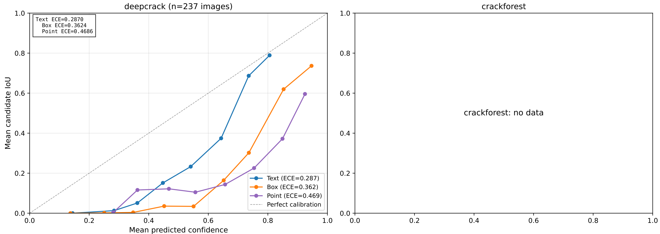
Figure S1 — Confidence Calibration Reliability Diagram
