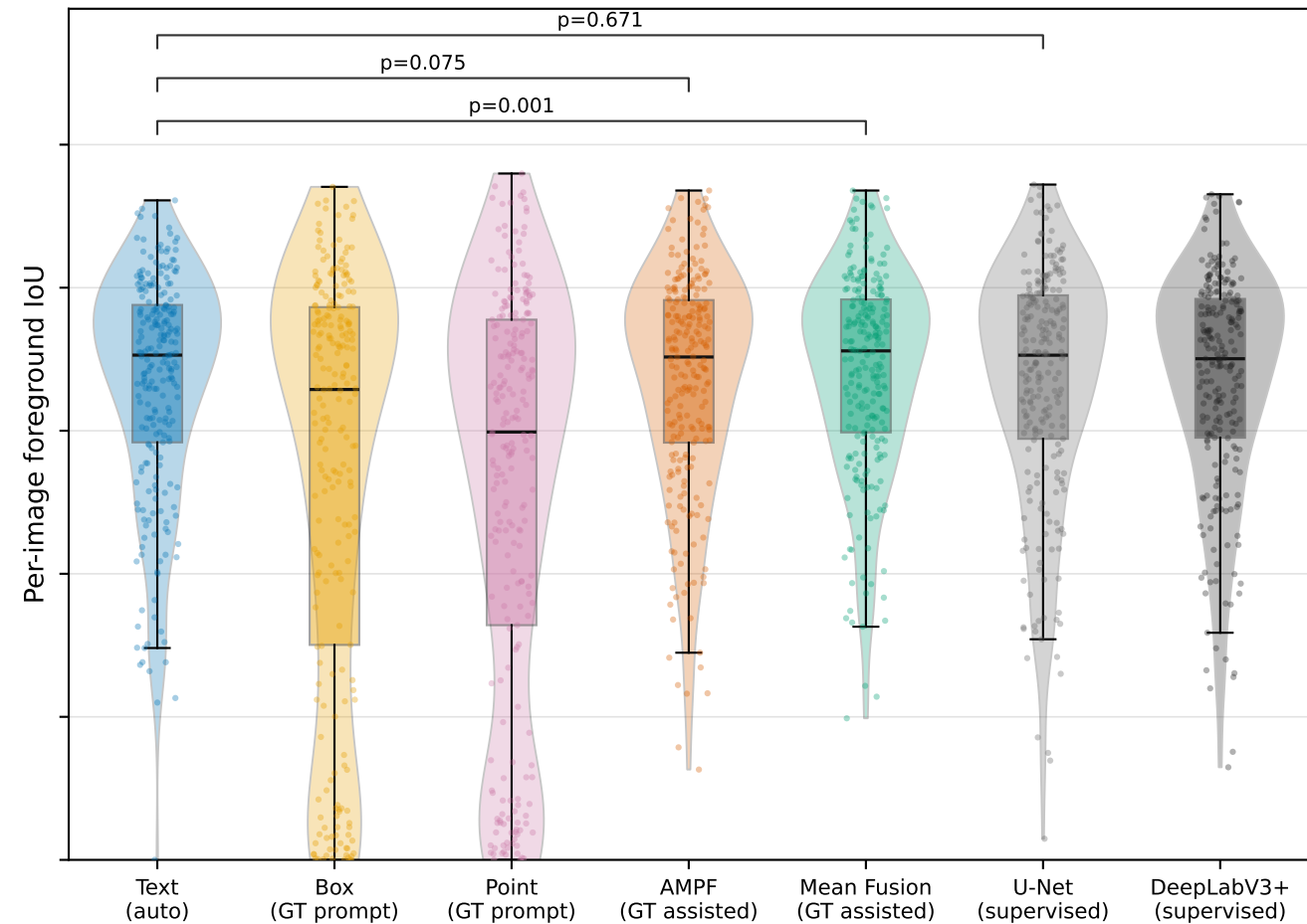
DeepCrack (n=237)
