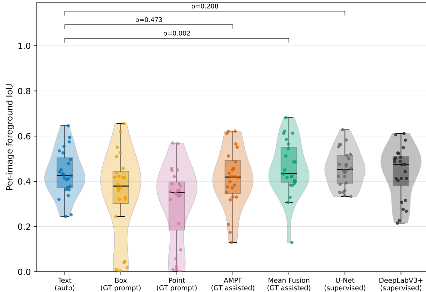
CrackForest (n=24)
