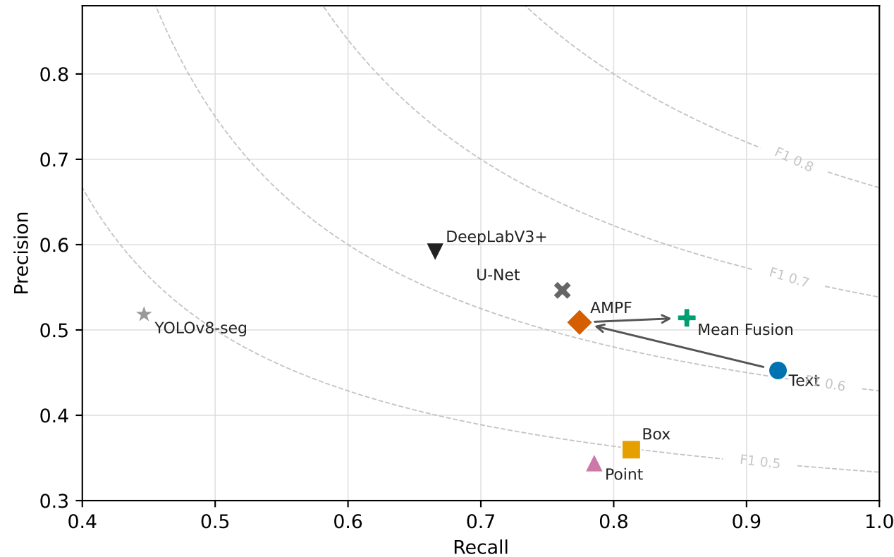
CrackForest
