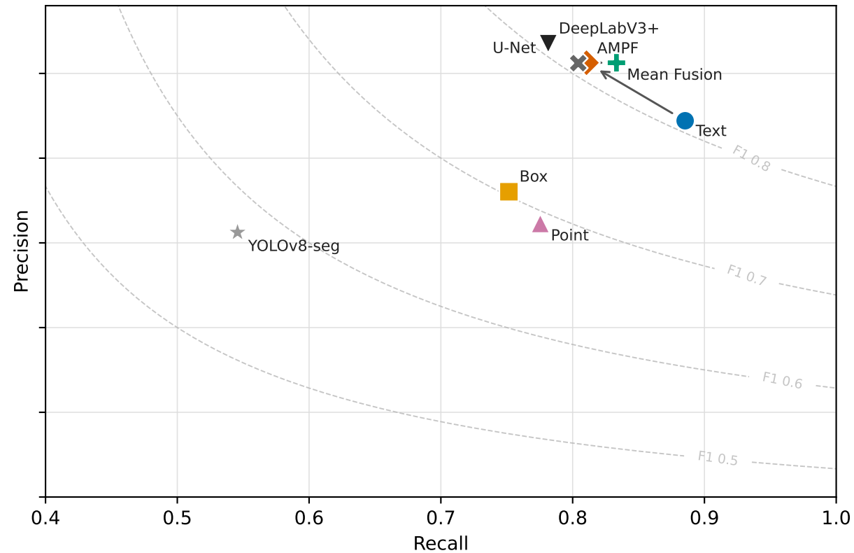
DeepCrack
