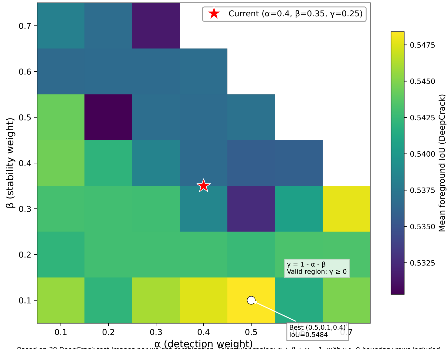
Figure S2 — AMPF Weight Sensitivity (DeepCrack)
