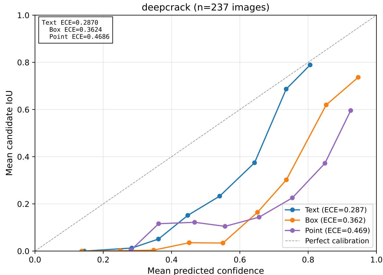
Figure S1 — Confidence Calibration Reliability Diagram
