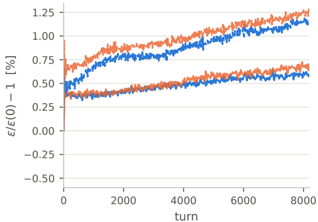
(b) proton, undamped
