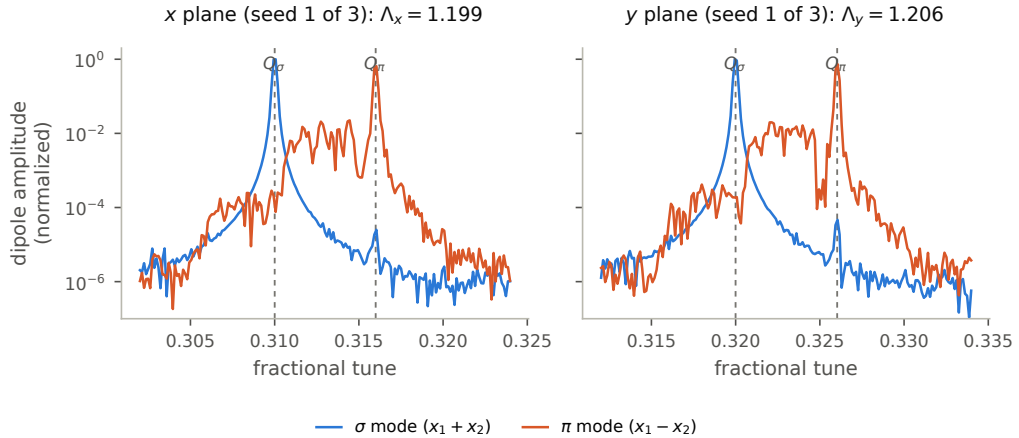
Figure 3: Round-beam PIC centroid spectra for one of three seeds (8192 turns, 10^5 macroparticles/beam, \xi = 0.005 , one slice). Each plane is normalized to its largest sum- or difference-mode amplitude. Dashed lines mark the fitted Q_\sigma and Q_\pi ; the other seeds give the scatter in Table 3.
