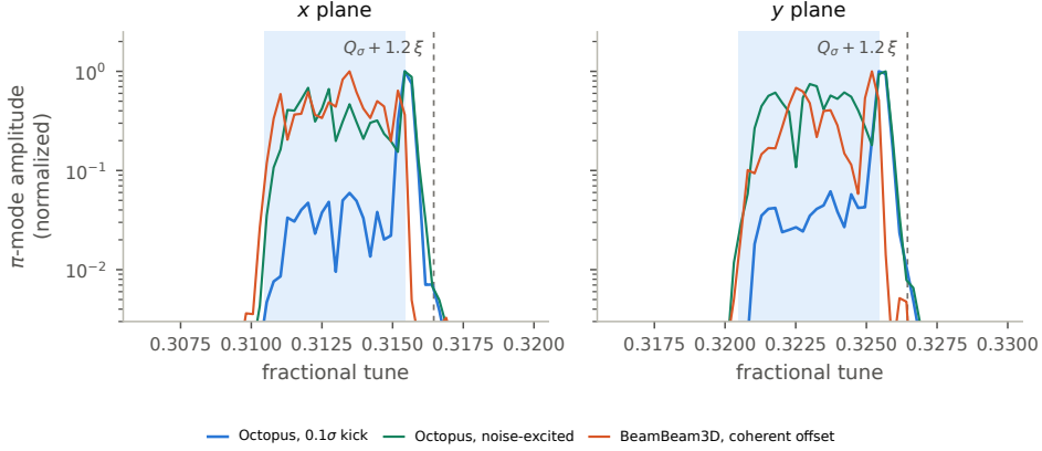
Figure 4: Five-slice normalized difference-mode spectra ( 5 \times 10^4 macroparticles/beam, \sigma_z/\beta^* = 0.5 , |Q_s| = 0.01 , \xi = 0.005 , 4096 turns). Shading spans [Q_\sigma, Q_\sigma + \xi] and the dashed line marks Q_\sigma + 1.2\xi . The noise-excited Octopus and coherently kicked BeamBeam3D horizontal traces each contain six peaks under the stated estimator; the comparison supports similar structure, not common mode identities.
