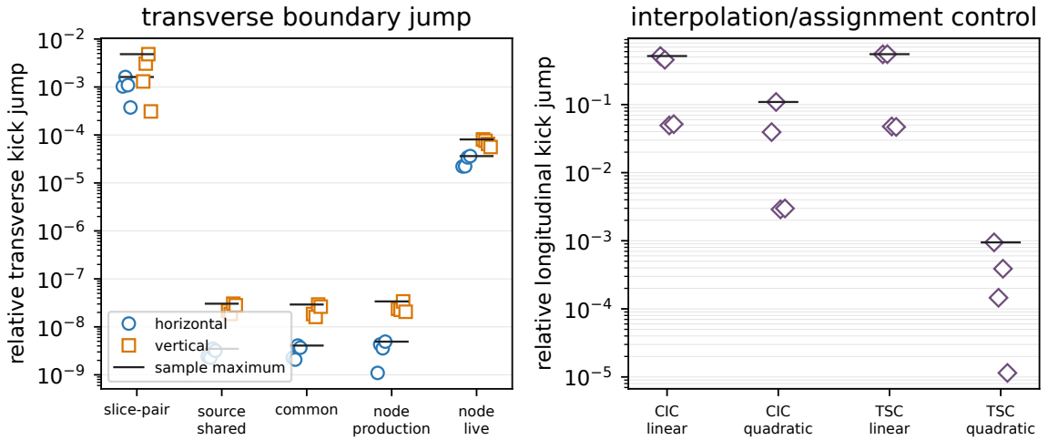
Figure 2: Slice-boundary tests for a flat EIC-like source, seven quantile slices, 64^2 cells, and 2 \times 10^5 macroparticles. Each jump is divided by the peak magnitude of the corresponding exact kick over the scan. (a) Four frozen-source grid constructions and a node-indexed live-source control; each marker is one of two source slices at one of two central boundaries. The “node production” values use the full scheduled node calculation. (b) Frozen-source longitudinal jumps for four assignment/interpolation combinations. Diamonds are the same four samples and horizontal bars mark their maxima.
