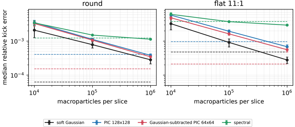
Figure 1: Median transverse-kick error relative to the peak exact kick for a round source and an 11:1 flat source, evaluated at 81^2 probes over \pm 4\sigma . Symbols and bars are means and sample standard deviations over six independent batch medians; each batch contains five paired source draws at 10^4 and 10^5 macroparticles and three at 10^6 . Dashed lines are deterministic-source estimates from a 400^2 Gaussian quantile lattice and contain source-quadrature as well as solver error; they are not bounds. PIC uses 128^2 cells, Gaussian-subtracted PIC 64^2 , and the independent spectral grids are 127^2 (round) and 127 \times 383 (flat), with domain half-width factors 16 and 8 relative to the larger measured source rms.
