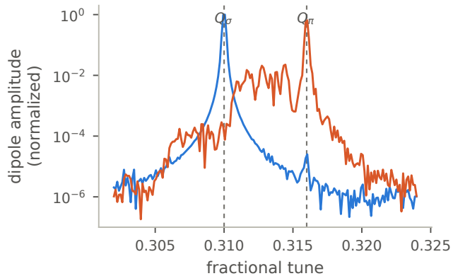
x plane (seed 1 of 3): \Lambda_x = 1.199
