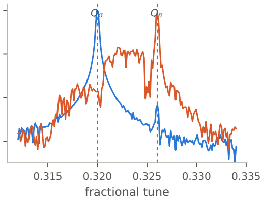
y plane (seed 1 of 3): \Lambda_y = 1.206
