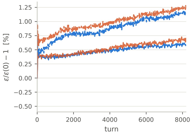
(b) proton, undamped
