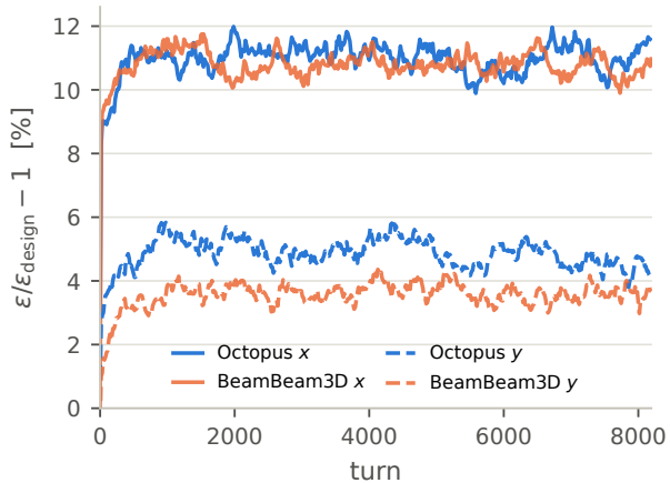
(a) electron, damped ( \tau = 400 turns)
