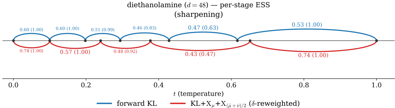
Figure 13: Diethanolamine per-stage ESS as annealing-ladder arcs (sharpening schedule): forward KL above the axis (blue), \text{KL} + \text{X}_\mu + \text{X}_{(\hat{\mu} + \bar{\nu})/2} , \delta -reweighted, below (red). Each arc is an accepted stage; the apex label is that stage’s validation ESS, with the sharpening ESS in parentheses.
