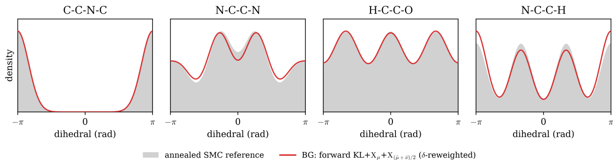
Figure 16: Alanine dipeptide torsion marginals of the BG deliverable (red) against a converged annealed SMC reference (grey). The four most multimodal proper torsions are shown; the densities are \pm\phi -symmetrised, the achiral target having p(\phi) = p(-\phi) . The BG recovers the multimodal backbone torsions and tracks the reference; the peptide-bond torsion \omega (C-C-N-C) is trans-dominant in the generator, the one torsion whose high rotation barrier also makes the uniform-init annealed SMC reference slow to converge.
