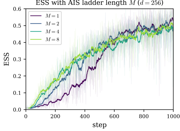
Figure 4: ESS trajectory across training steps for the mixture loss \text{KL}+X_\mu+X_{(\hat{\mu}+\hat{\nu})/2} on the product multi-well at d = 256 , as the AIS ladder length M that builds the \mu -surrogate is varied over \{1, 2, 4, 8\} . Faint lines are the raw per-step ESS; bold lines are a moving average.
