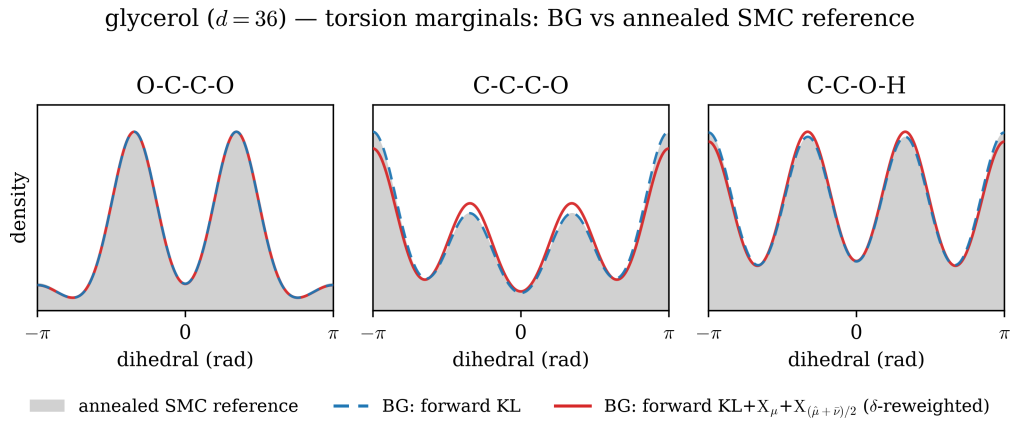
Figure 12: Glycerol torsion marginals of both generators against a converged annealed SMC reference (grey): forward KL (blue) and \text{KL} + X_\mu + X_{(\hat{\mu} + \bar{\nu})/2} , \delta -reweighted (red), both sharpened with the cap annealed to e_{\text{cap}} = 200 kJ/mol. Both recover the multimodal gauche ^\pm /trans structure of the characteristic glycerol torsions.
