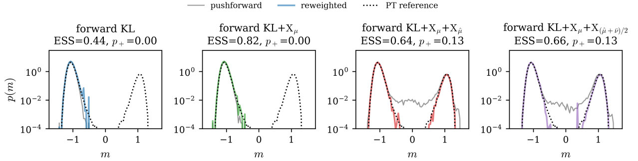
Figure 5: Magnetization density p(m) on the L = 8 lattice, one panel per training loss. Each panel shows the pushforward density (gray), the reweighted density (color), and the PT reference (dotted); the title reports the final ESS and the reweighted p_+ .
