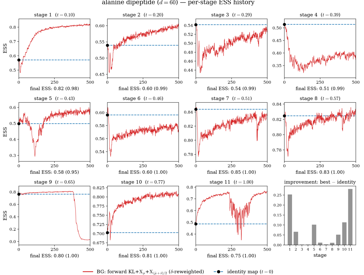
Figure 15: Alanine dipeptide per-stage ESS history: each panel is the per-step effective sample size during that stage’s X-regularized \delta -reweighted flow training (red), against the identity-map baseline at t = 0 (blue dashed). Below each panel is that stage’s accepted validation ESS with the sharpening ESS in parentheses. The dip across t \approx 0.29 – 0.43 is the clash bottleneck, with ESS recovering to \approx 0.8 once the cap is sharp enough to separate the basins.
