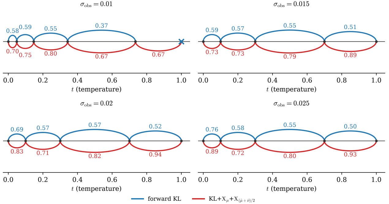
Figure 10: ESS ladders on the screened Poisson posterior across the noise sweep, one panel per \sigma_{\text{obs}} . The temperature axis runs t = 0 \rightarrow 1 ; each accepted stage is an arc spanning its increment \Delta t_k , forward KL above (blue) and the X-regularized loss \text{KL} + X_\mu + X_{(\hat{\mu} + \bar{\nu})/2} below (red), labelled by its per-stage validation ESS. The cross marks the final bridge that the forward KL run failed in all ten attempts at \sigma_{\text{obs}} = 0.01 . The recovered well weights are reported in Table 7.
