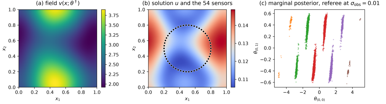
Figure 9: The screened Poisson inverse problem. (a) The field v(\mathbf{x}; \theta^\dagger) on [0, 1]^2 , whose cosine modulation 3(1 + \frac{1}{2} \cos(3v(\mathbf{x}; \theta^\dagger))) is the source. (b) The corresponding solution u of (19) and the 54 sensors on the ring of radius 0.3, the dotted circle, where u is observed. (c) The marginal posterior in the coefficients (\theta_{(0,0)}, \theta_{(0,1)}) from the parallel tempering referee at \sigma_{\text{obs}} = 0.01 , colored by the shift index n : the posterior splits into the well lattice of the cosine symmetries.
