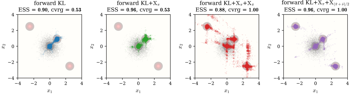
Figure 5: Sparse target. Columns show forward KL, KL+ X_\pi , KL+ X_\pi+X_{\hat{\pi}} , and KL+ X_\pi+X_{(\hat{\pi}+\bar{\nu})/2} , with the pushforward samples overlaid on the target energy; panel titles report final ESS and coverage, and gray points show the source.
