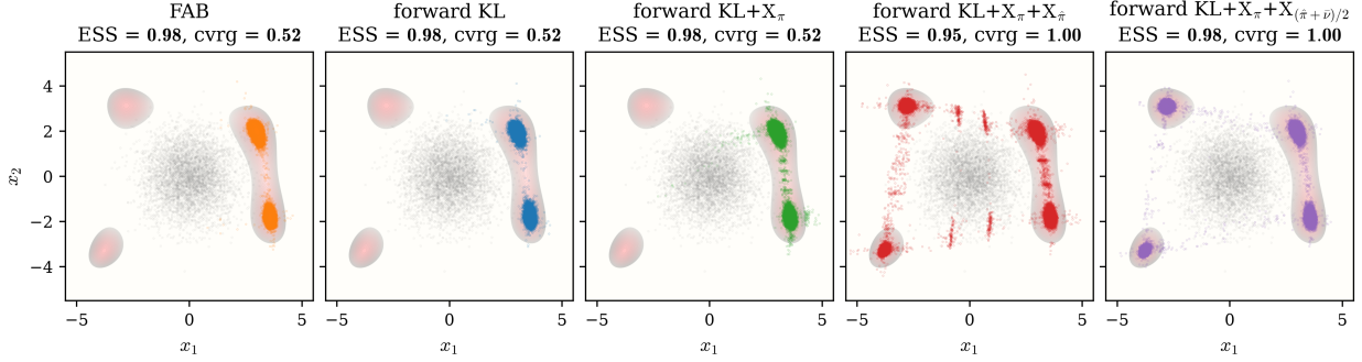
Figure 4: Himmelblau target. Columns show FAB, forward KL, KL+ X_\pi , KL+ X_\pi + X_{\hat{\pi}} , and KL+ X_\pi + X_{(\hat{\pi}+\bar{\nu})/2} ; each panel shows the pushforward samples over the target energy with final ESS and coverage, and gray points show the source.
