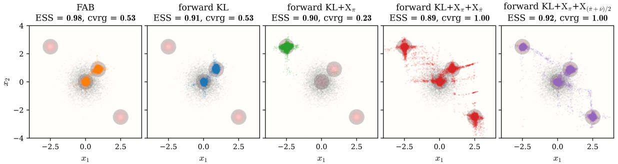
Figure 5: Sparse target. Columns show FAB, forward KL, KL+ X_\pi , KL+ X_\pi + X_{\hat{\pi}} , and KL+ X_\pi + X_{(\hat{\pi}+\bar{\nu})/2} , with the pushforward samples overlaid on the target energy; panel titles report final ESS and coverage, and gray points show the source.
