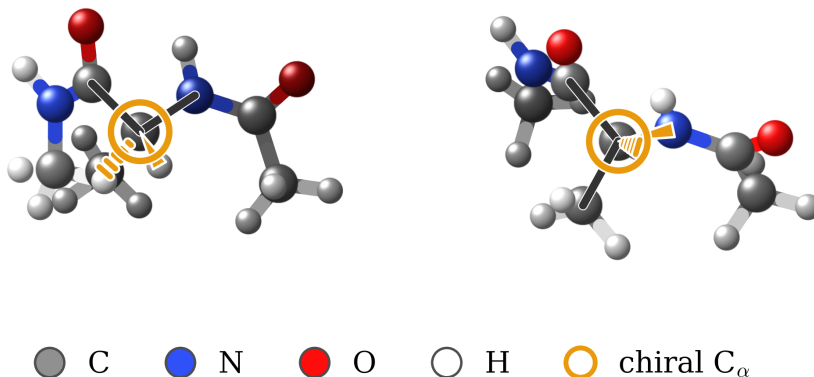
Figure 21: The two enantiomers of alanine dipeptide: the energy-minimized L-form and the D-form, a 3D reflection of it, shown from different viewpoints (ball-and-stick; C grey, N blue, O red, H white). The chiral C_\alpha is ringed in gold with stereo bonds, a solid wedge toward the viewer and hashed bonds behind. The achiral Amber force field makes the two isoenergetic, so the generator emits both, the structural companion to the (\phi, \psi) \rightarrow (-\phi, -\psi) Ramachandran symmetry of Figure 22.
