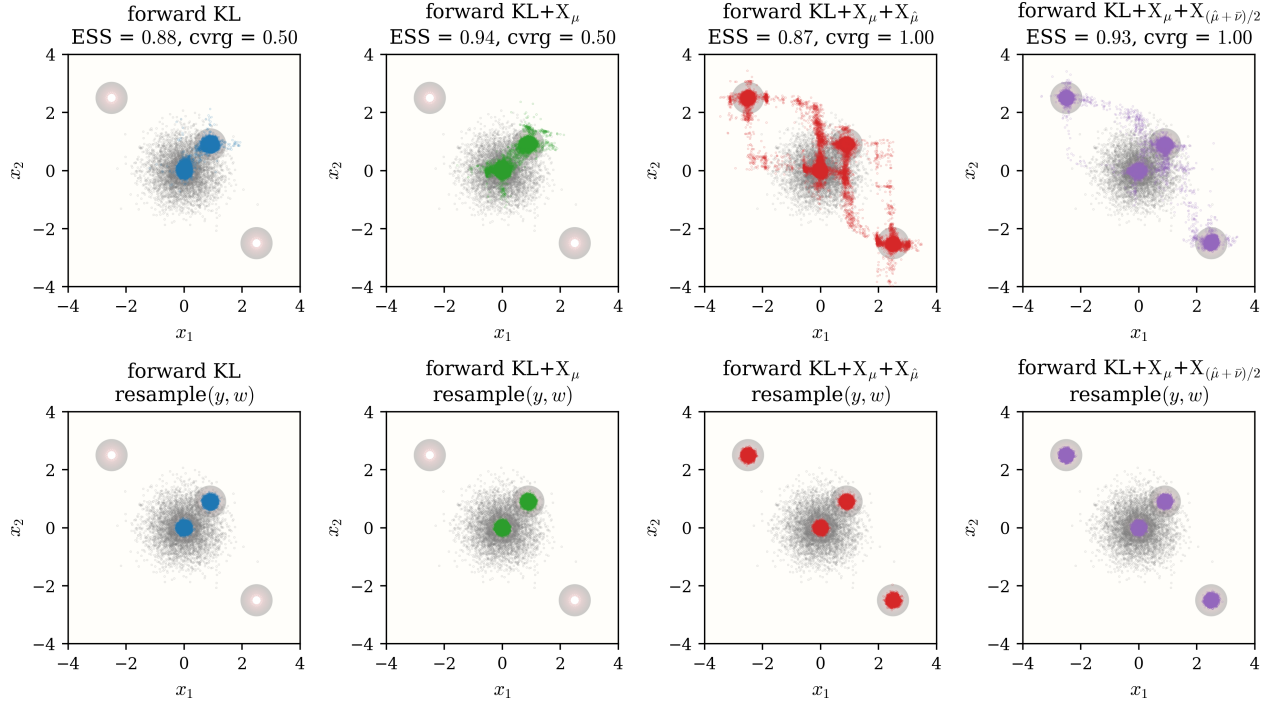
Figure 4: Sparse target. Row 1: pushforward \mathbf{y} = G^{-1}(\mathbf{x}) . Row 2: resample( \mathbf{y}, w ) with Langevin rejuvenation. Columns as in Figure 1.
