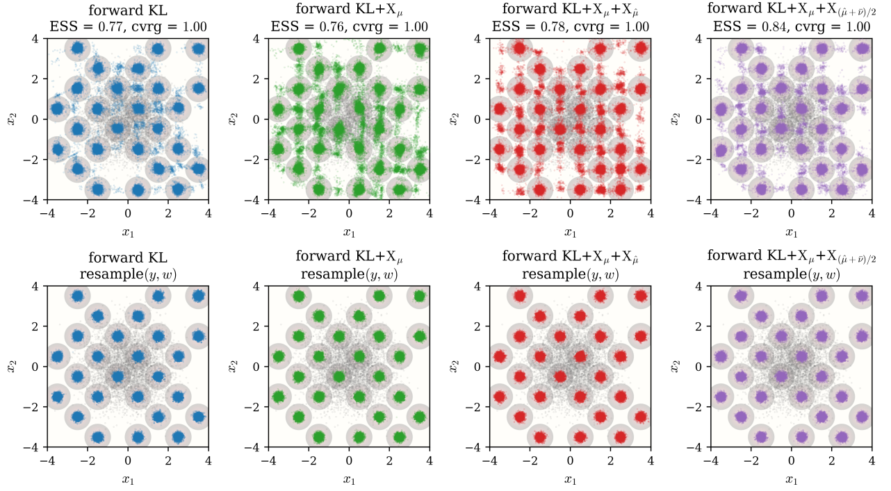
Figure 3: Chessboard target. Row 1: pushforward \mathbf{y} = G^{-1}(\mathbf{x}) . Row 2: resample( \mathbf{y}, w ) with Langevin rejuvenation. Columns as in Figure 1.
