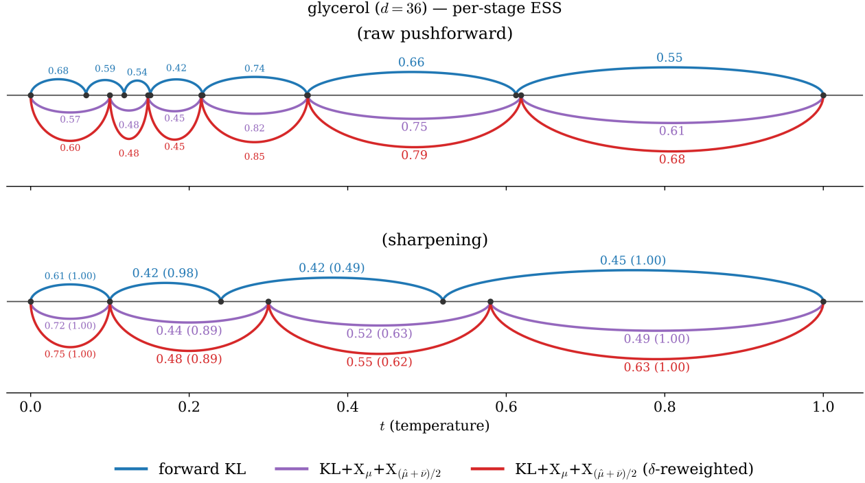
Figure 11: Glycerol per-stage validation ESS as annealing-ladder arcs, raw (top) and sharpen (bottom). In each row forward KL is drawn above the axis (blue), \text{KL} + X_\mu + X_{(\hat{\mu} + \hat{\nu})/2} below (purple), and its \delta -reweighted variant further below (red). Each arc is an accepted stage; the apex label is that stage’s validation ESS; a cross marks a bridge the ladder failed to reach.
