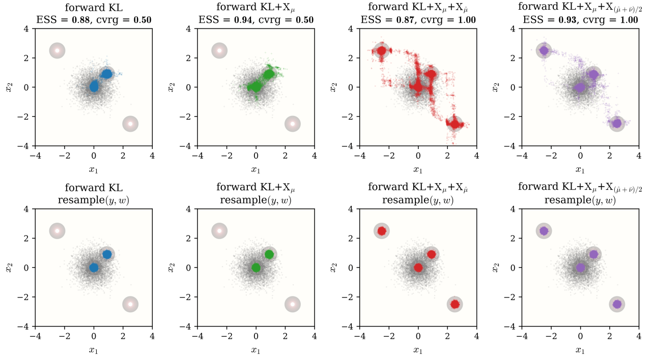
Figure 3: Sparse target. Row 1: pushforward \mathbf{y} = G^{-1}(\mathbf{x}) . Row 2: \text{resample}(\mathbf{y}, w) with Langevin rejuvenation. Columns as in Figure 1.
