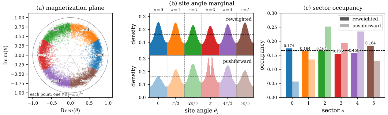
Figure 6: Structure of the cold clock measure (20) at d=64 , displayed on 10^6 reweighted samples: fresh source draws advanced through the trained ladder by the map–reweight–resample step (v), X-regularized loss at B=10^4 . (a) Global magnetization m(\theta) , colored by sector index s(\theta) , 1500 points per sector: the measure splits into p=6 equivalent sectors with mean |m|=0.73 . (b) Site-angle marginal: the anisotropy locks each site to the six clock angles 2\pi s/6 , s=0, \dots, 5 ; dashed lines bound the six wells, colored as in (c), and the black line marks the uniform density \frac{1}{2\pi} . The pushforward marginal is from the maps alone, without reweighting. (c) Sector occupancy of reweighted and pushforward samples, the black line marking the uniform occupancy \frac{1}{6} .
