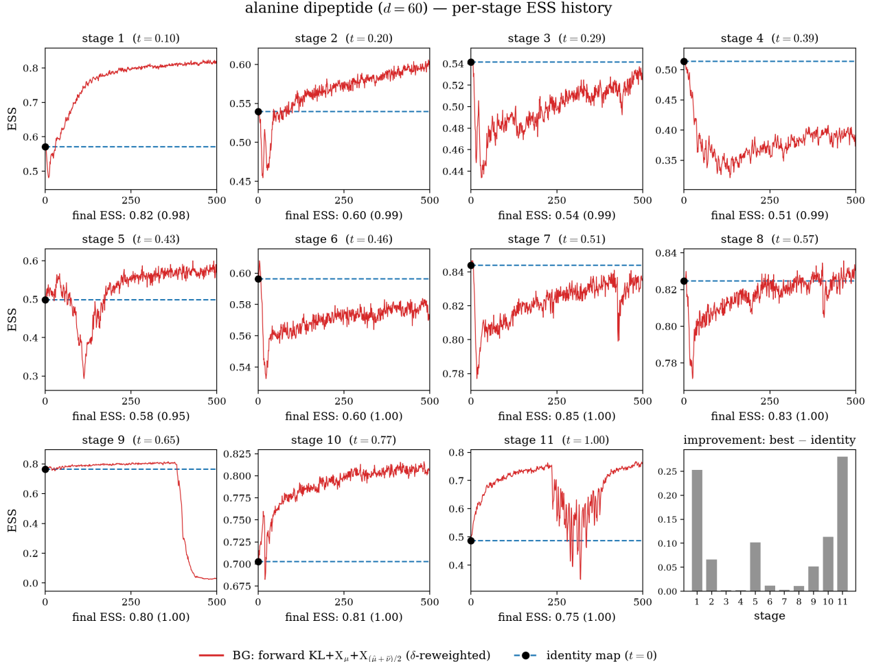
Figure 15: Alanine dipeptide per-stage ESS history: each panel is the per-step effective sample size during that stage’s X-regularized \delta -reweighted flow training (red), against the identity-map baseline at t = 0 (blue dashed). Below each panel is that stage’s accepted validation ESS with the sharpening ESS in parentheses. The dip across t \approx 0.29 – 0.43 is the clash bottleneck, with ESS recovering to \approx 0.8 once the cap is sharp enough to separate the basins.
