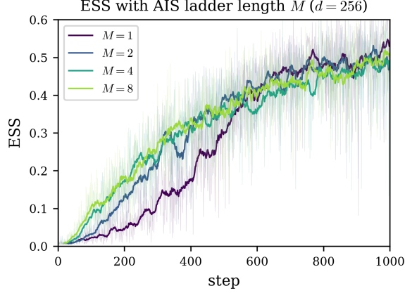
Figure 4: ESS trajectory across training steps for the mixture loss \text{KL}+X_\mu+X_{(\hat{\mu}+\hat{\nu})/2} on the product multi-well at d=256 , as the AIS ladder length M that builds the \mu -surrogate is varied over \{1, 2, 4, 8\} . Faint lines are the raw per-step ESS; bold lines are a moving average.
