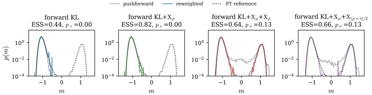
Figure 5: Magnetization density p(m) on the L=8 lattice, one panel per training loss. Each panel shows the pushforward density (gray), the reweighted density (color), and the PT reference (dotted); the title reports the final ESS and the reweighted p_+ .
