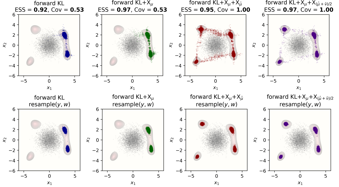
Figure 1: Himmelblau target. Row 1: pushforward y = G^{-1}(x) . Row 2: \text{resample}(y, w) with Langevin rejuvenation. Columns left to right: forward KL, +X_\mu , +X_\mu + X_{\hat{\mu}} , +X_\mu + X_{(\hat{\mu} + \bar{v})/2} . Each pushforward panel title reports the final ESS and the k = 5 coverage against \hat{\mu} .
