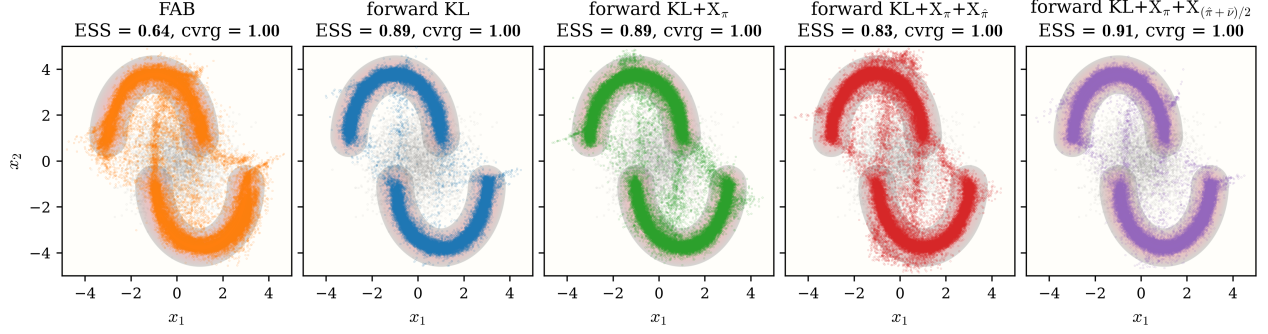
Figure 2: Two-Moon target. Columns, from left to right, are FAB, forward KL, KL+ X_\pi , KL+ X_\pi+X_{\hat{\pi}} , and KL+ X_\pi+X_{(\hat{\pi}+\bar{\nu})/2} . Each panel overlays the pushforward samples on the target energy and reports final ESS and coverage. Gray points show the source.
