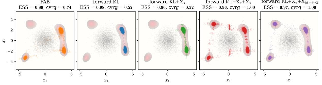
Figure 4: Himmelblau target. Columns show FAB, forward KL, KL+ X_\pi , KL+ X_\pi + X_{\hat{\pi}} , and KL+ X_\pi + X_{(\hat{\pi}+\bar{\nu})/2} ; each panel shows the pushforward samples over the target energy with final ESS and coverage, and gray points show the source.
