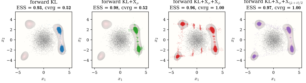
Figure 3: Himmelblau target. Columns show forward KL, \text{KL}+X_\mu , \text{KL}+X_\mu+X_{\hat{\mu}} , and \text{KL}+X_\mu+X_{(\hat{\mu}+\hat{\nu})/2} ; each panel shows the pushforward samples over the target energy with final ESS and coverage, and gray points show the source. The first two objectives capture only two of the four wells. Both \hat{\mu} -weighted objectives cover all four, while including pushforward samples in the mixture term reduces the visible intermodal mass and raises ESS relative to the \text{KL}+X_\mu+X_{\hat{\mu}} fit.
