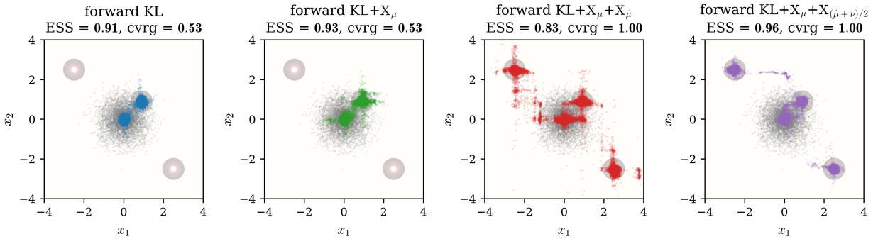
Figure 4: Sparse target. Columns show forward KL, \text{KL}+X_\mu , \text{KL}+X_\mu+X_{\hat{\mu}} , and \text{KL}+X_\mu+X_{(\hat{\mu}+\hat{\nu})/2} , with the pushforward samples overlaid on the target energy; panel titles report final ESS and coverage, and gray points show the source. The first two objectives cover the central pair but miss the two remote modes. The loss \text{KL}+X_\mu+X_{\hat{\mu}} restores the remote modes with visible mass between components, whereas the equal mixture covers all four modes with less intermodal mass and higher ESS.
