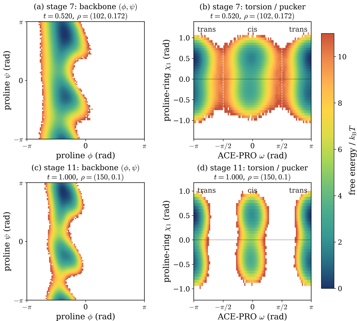
Figure 16: Conformational free energy surfaces for Ac-Pro-NHMe from 1.5 \times 10^7 inference samples per stage. The upper row is stage 7, the accepted stage nearest t = 0.5 , at t = 0.520 and \rho = (102, 0.172) ; the lower row is the final stage 11 at t = 1 and \rho = (150, 0.10) . The left column shows the proline backbone (\phi, \psi) surface, and the right column shows the joint ACE-PRO peptide torsion \omega and proline-ring pucker \chi_1 , with the cis and trans sectors marked. All four panels share one free energy scale in units of k_B T .
