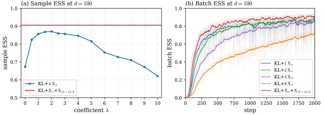
Figure 7: Effect of the target-variation coefficient on the product multi-well target (32) at d = 100 . (a) Final sample ESS of \text{KL} + \lambda X_{\pi} against \lambda ; the horizontal line is the KLXX value 0.906. The sweep runs from 0.673 at \lambda = 0 through its maximum 0.871 at \lambda = 2 to 0.622 at \lambda = 10 . (b) Batch ESS during training at \lambda = 1, 2, 4, 8 and for KLXX; bold curves are 40-step moving averages of the raw values.
