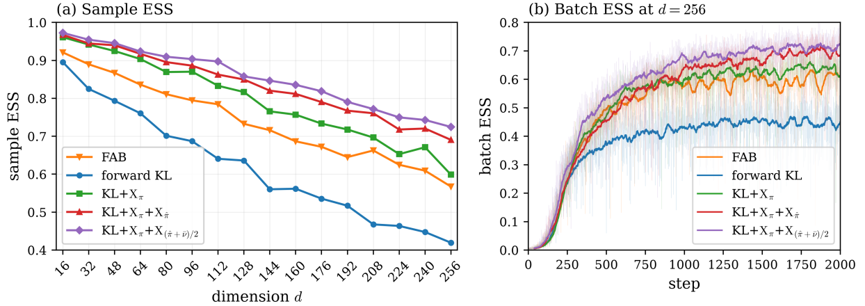
Figure 6: ESS on the product multi-well target (32). (a) Final sample ESS over sixteen tested dimensions. At d = 256 the values are 0.419 for forward KL, 0.567 for FAB, 0.599 for KL+X _{\pi} , 0.690 for KL+X _{\pi} +X _{\hat{\pi}} , and 0.725 for KLXX. (b) Batch ESS during the d = 256 training; bold curves are 40-step moving averages of the raw values.
