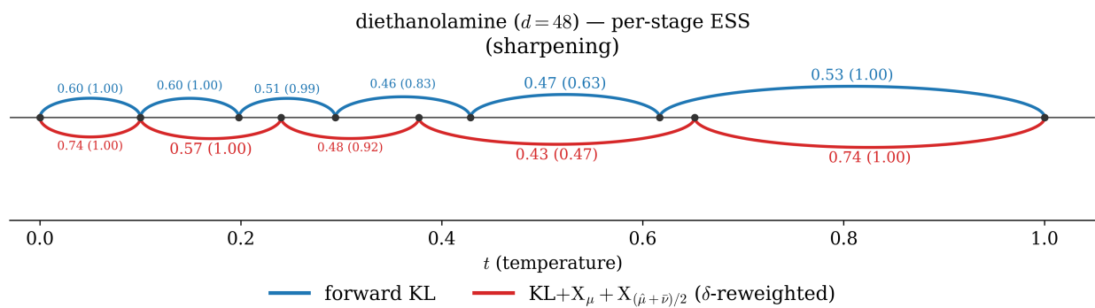
Figure 16: Diethanolamine per-stage ESS as annealing-ladder arcs (sharpening schedule): forward KL above the axis (blue), \text{KL} + X_\mu + X_{(\mu+\bar{\nu})/2} , \delta -reweighted, below (red). Each arc is an accepted stage; the apex label is that stage's validation ESS, with the sharpening ESS in parentheses.
