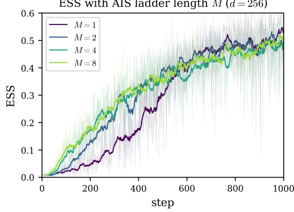
Figure 6: ESS trajectory across training steps for the mixture loss \text{KL}+X_\mu+X_{(\hat{\mu}+\bar{v})/2} on the product multi-well at d = 256 , as the AIS ladder length M that builds the \mu -surrogate is varied over \{1, 2, 4, 8\} . Faint lines are the raw per-step ESS; bold lines are a moving average.
