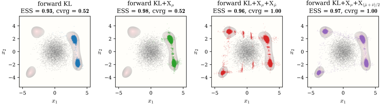
Figure 3: Himmelblau target. Columns show forward KL, \text{KL} + X_\mu , \text{KL} + X_\mu + X_{\hat{\mu}} , and \text{KL} + X_\mu + X_{(\hat{\mu} + \hat{\nu})/2} ; each panel shows the pushforward over the target energy with final ESS and coverage, and gray points show the source. The first two objectives capture only two of the four wells. Both \hat{\mu} -weighted objectives cover all four, while including pushforward samples in the mixture term reduces the visible intermodal mass and raises ESS relative to the \hat{\mu} -only fit.
