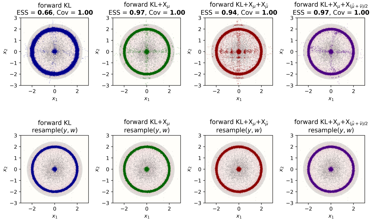
Figure 2: Annulus target. Row 1: pushforward y = G^{-1}(x) . Row 2: \text{resample}(y, w) with Langevin rejuvenation. Columns as in Figure 1.
