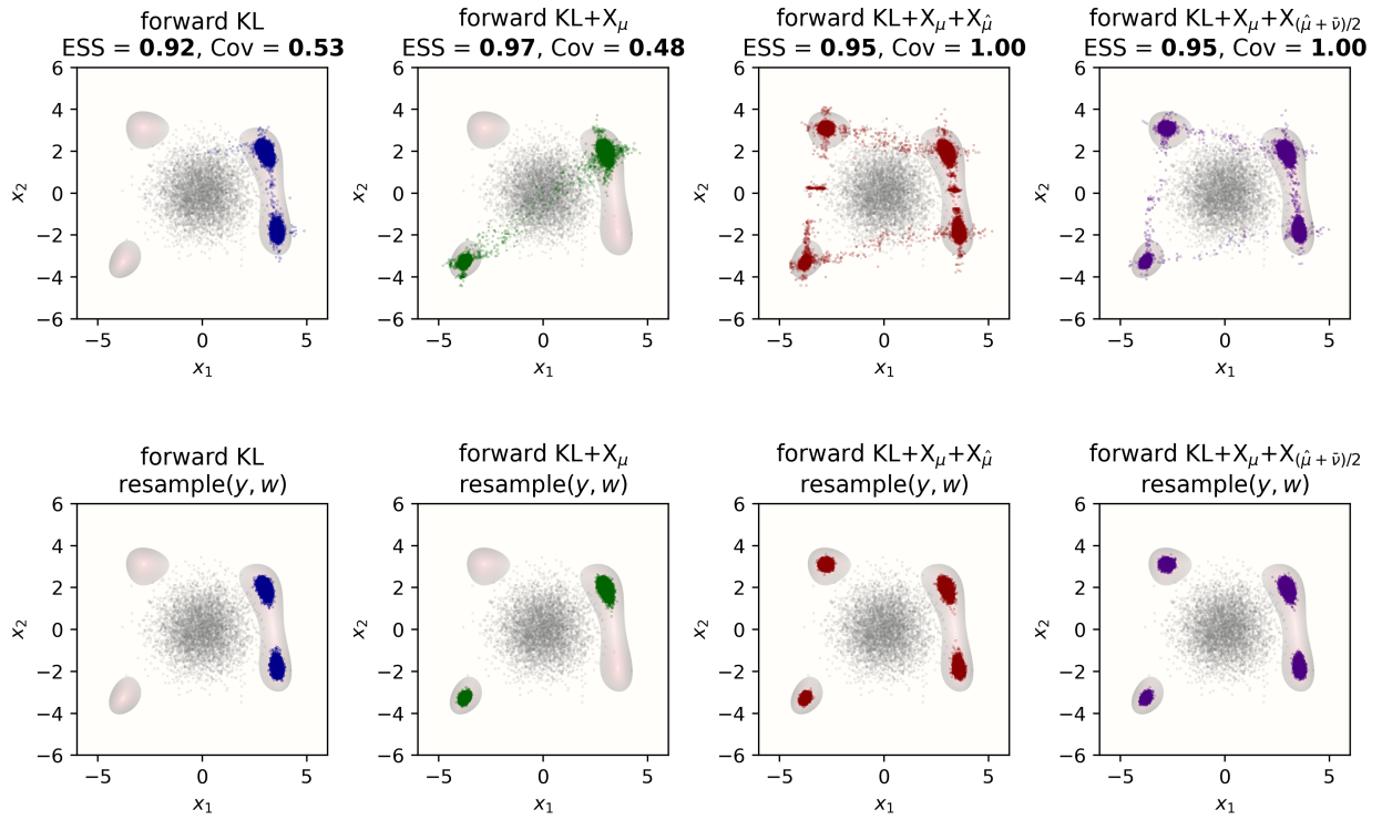
Figure 1: Himmelblau target. Row 1: pushforward y = G^{-1}(x) . Row 2: resample( y, w ) with Langevin rejuvenation. Columns left to right: forward KL, KL+ X_\mu , KL+ X_\mu + X_{\hat{\mu}} , KL+ X_\mu + X_{(\hat{\mu} + \bar{v})/2} . Each pushforward panel title reports the final ESS and the k = 5 coverage against \hat{\mu} .
