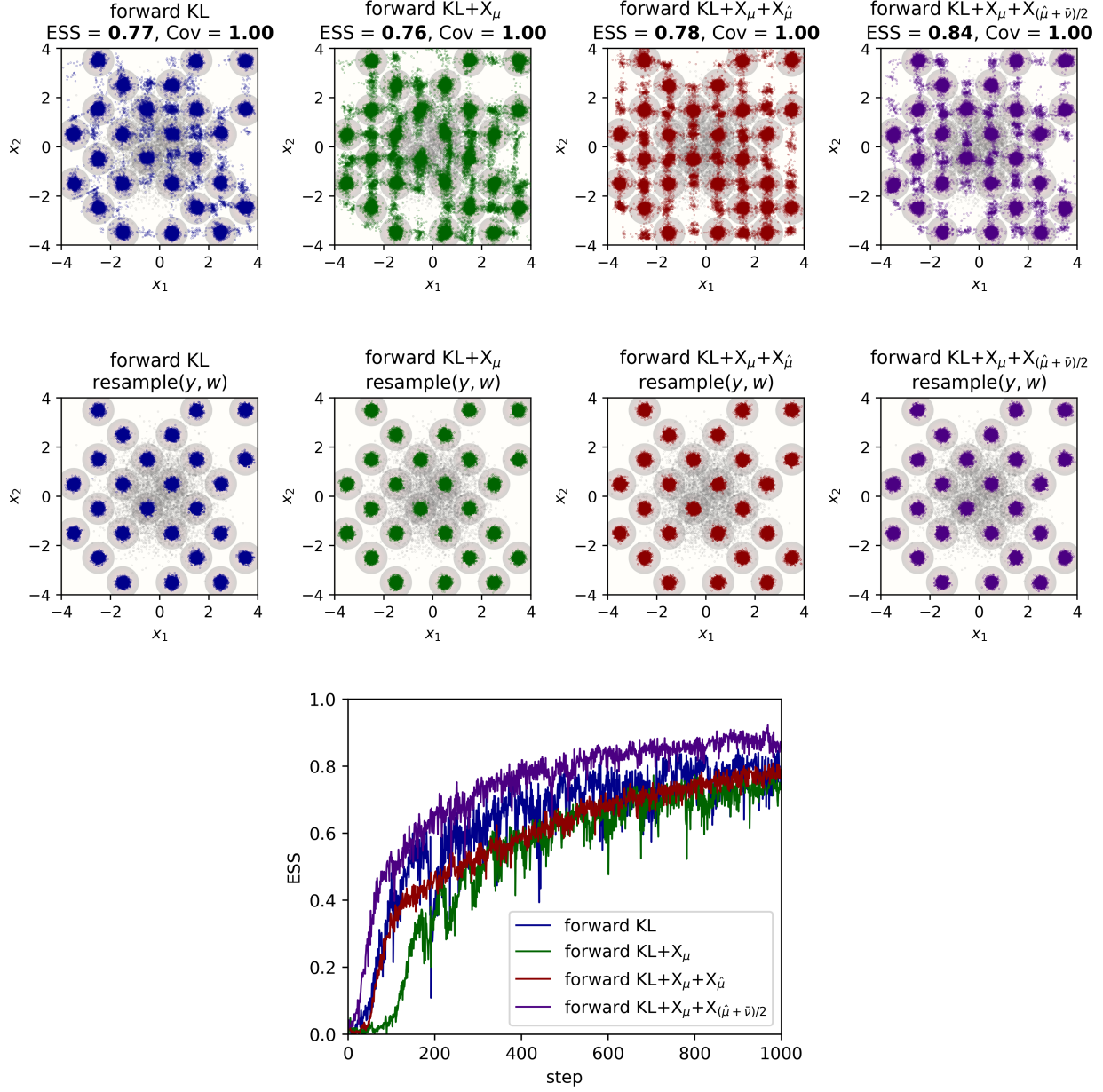
Figure 4: Chessboard target. Row 1: pushforward y = G^{-1}(x) . Row 2: resample( y, w ) with Langevin rejuvenation. Columns as in Figure 1. Row 3: ESS trajectory across training steps – bare forward KL and KL+ X_\mu fluctuate strongly throughout training, while the wide-coverage X_{\hat{\mu}} and mixture variants settle into markedly steadier curves, with the mixture both the highest and the tightest.
