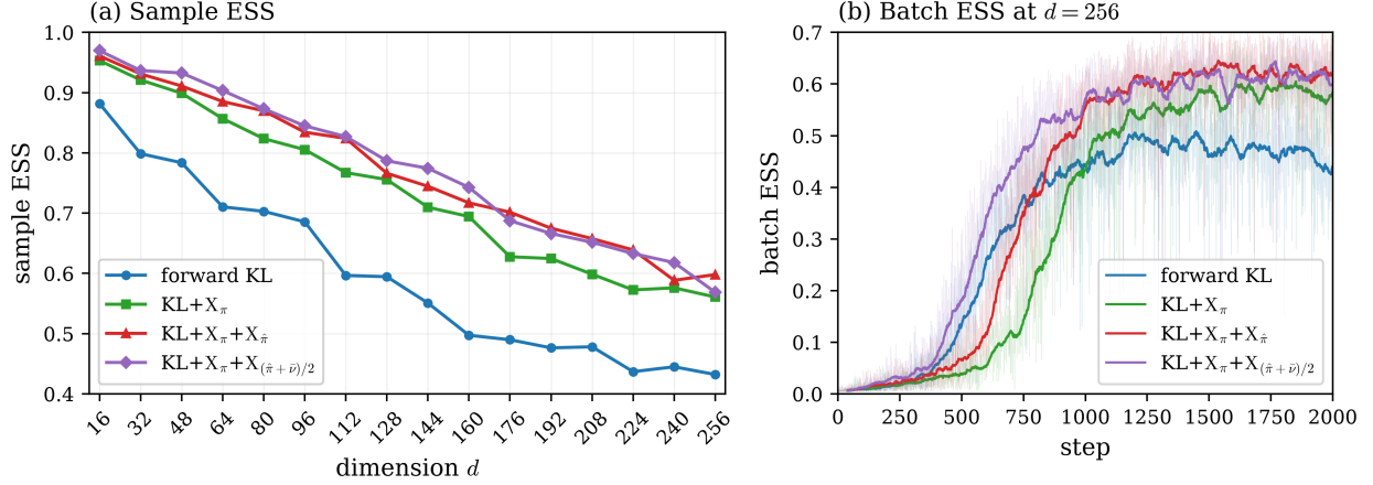
Figure 6: ESS on the product multi-well target (33). (a) Final sample ESS over sixteen tested dimensions. (b) Batch ESS during the d=256 training; bold curves are 40-step moving averages of the raw values.
