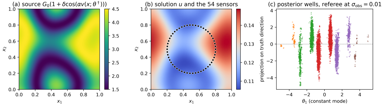
Figure 11: The screened Poisson inverse problem. (a) The true source G_0(1 + \delta \cos(\alpha v(x; \theta^\dagger))) on [0, 1]^2 . (b) The corresponding solution u of (32) and the 54 sensors on the ring of radius 0.3, the dotted circle, where u is observed. (c) Posterior samples from the parallel tempering referee at \sigma_{\text{obs}} = 0.01 , plotted in the constant mode \theta_1 against the projection on the truth direction and colored by the shift index n : the posterior splits into the well lattice of the cosine symmetries, the structure the ladder must reproduce with the correct relative weights.
