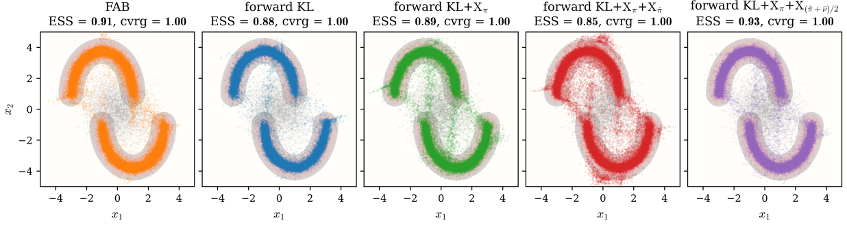
Figure 2: Two-Moon target. Columns, from left to right, are FAB, forward KL, KL+ X_\pi , KL+ X_\pi + X_{\hat{\pi}} , and KL+ X_\pi + X_{(\hat{\pi}+\bar{\nu})/2} . Each panel overlays the pushforward samples on the target energy and reports final ESS and coverage. Gray points show the source.
