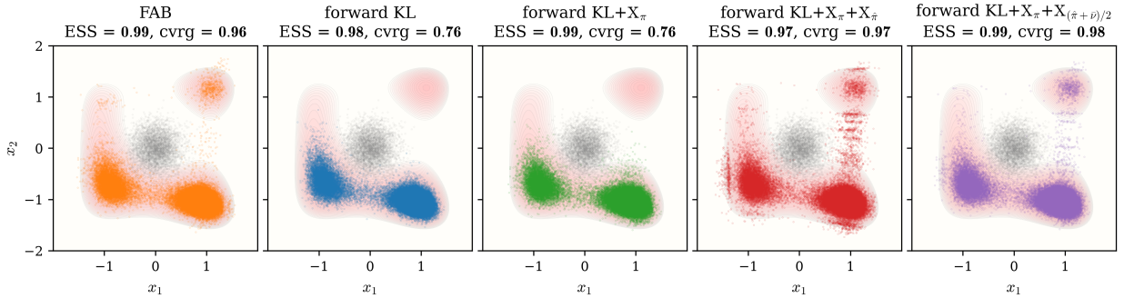
Figure 3: Three-Well target. From left to right, the panels show FAB, forward KL, KL+ X_\pi , KL+ X_\pi + X_{\hat{\pi}} , and KL+ X_\pi + X_{(\hat{\pi}+\bar{\nu})/2} . Each panel overlays the pushforward samples on the target energy and reports final ESS and coverage; gray points show the source.
