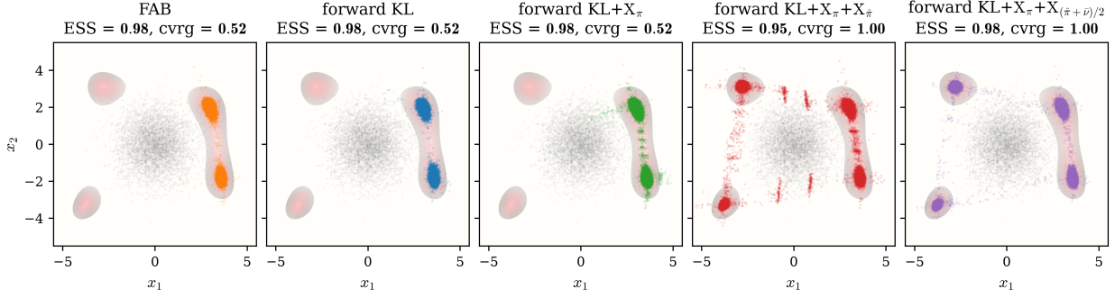
Figure 4: Himmelblau target. Columns show FAB, forward KL, \text{KL}+X_\pi , \text{KL}+X_\pi+X_{\hat{\pi}} , and \text{KL}+X_\pi+X_{(\hat{\pi}+\bar{\nu})/2} ; each panel shows the pushforward samples over the target energy with final ESS and coverage, and gray points show the source.
