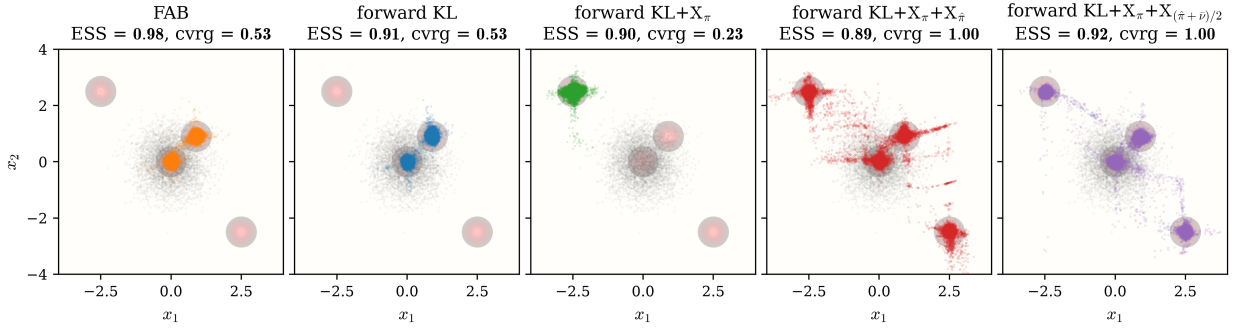
Figure 5: Sparse target. Columns show FAB, forward KL, \text{KL}+X_\pi , \text{KL}+X_\pi+X_{\hat{\pi}} , and \text{KL}+X_\pi+X_{(\hat{\pi}+\bar{\nu})/2} , with the pushforward samples overlaid on the target energy; panel titles report final ESS and coverage, and gray points show the source.
