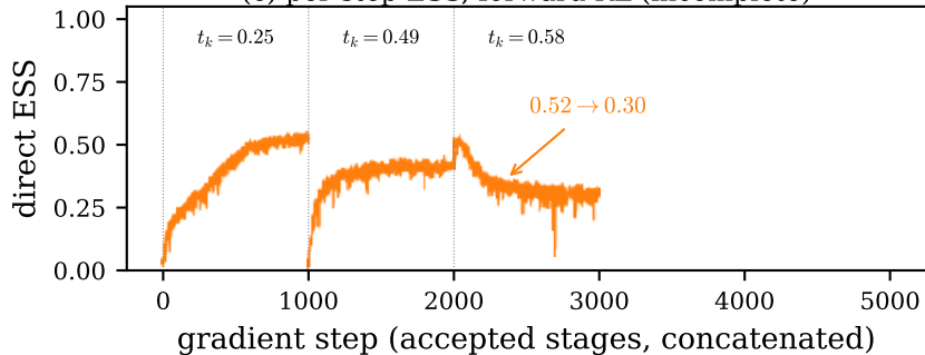
(c) per-step ESS, forward KL (incomplete)
