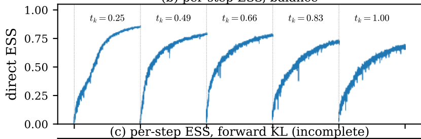
(b) per-step ESS, balance
