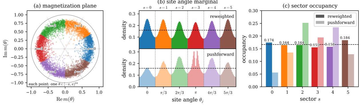
Figure 8: Structure of the cold clock measure (28) at d = 64 , displayed on 10^6 reweighted samples: fresh source draws advanced through the trained ladder by the map–reweight–resample step (v), X-regularized loss at B = 10^4 . (a) Global magnetization m(\theta) , colored by sector index s(\theta) , 1500 points per sector: the measure splits into p = 6 equivalent sectors with mean |m| = 0.73 . (b) Site-angle marginal: the anisotropy locks each site to the six clock angles 2\pi s/6 , s = 0, \dots, 5 ; dashed lines bound the six wells, colored as in (c), and the black line marks the uniform density \frac{1}{2\pi} ; the pushforward marginal is from the maps alone, without reweighting. (c) Sector occupancy of reweighted and pushforward samples, the black line marking the uniform occupancy \frac{1}{6} .
