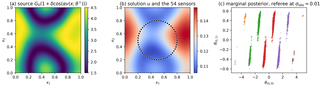
Figure 11: The screened Poisson inverse problem. (a) The true source 3(1 + \frac{1}{2}\cos(3v(\mathbf{x}; \theta^\dagger))) on [0, 1]^2 . (b) The corresponding solution u of (29) and the 54 sensors on the ring of radius 0.3, the dotted circle, where u is observed. (c) The marginal posterior in the coefficients (\theta_{(0,0)}, \theta_{(0,1)}) from the parallel-tempering referee at \sigma_{\text{obs}} = 0.01 , colored by the shift index n : the posterior splits into the well lattice of the cosine symmetries.
