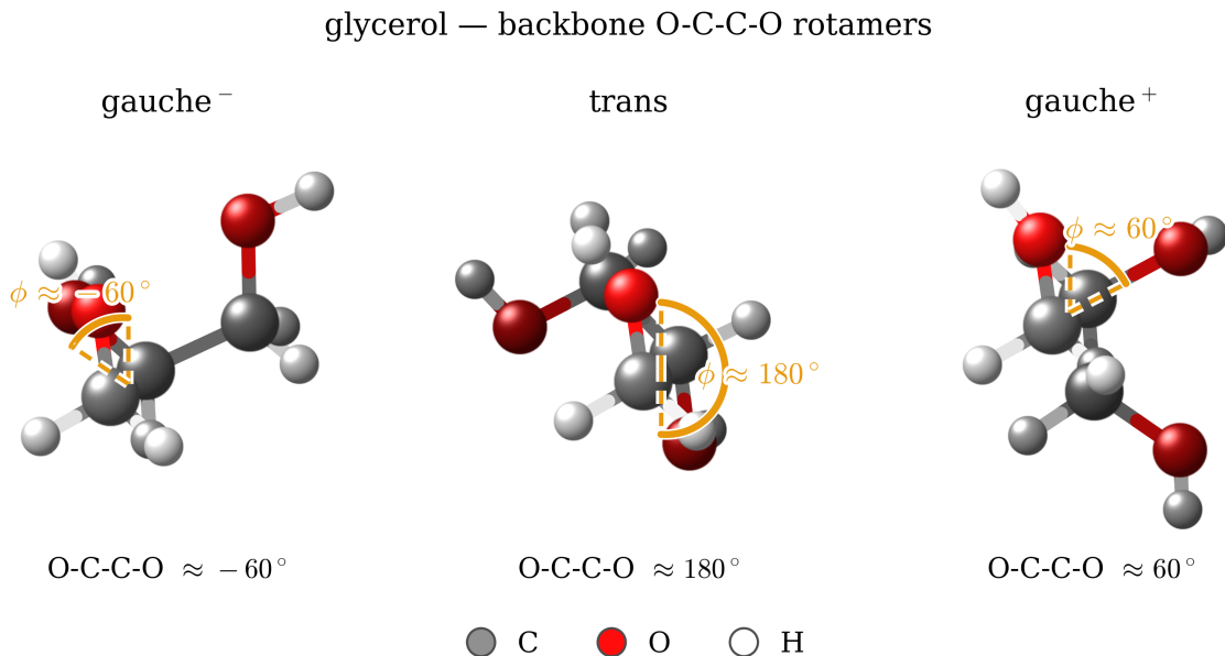
Figure 14: Typical glycerol configurations at the three states of the backbone O-C-C-O torsion: gauche − ( -60^\circ ), trans ( 180^\circ ), gauche + ( +60^\circ ). The gold arc marks the dihedral \phi ; ball-and-stick (C grey, O red, H white).
