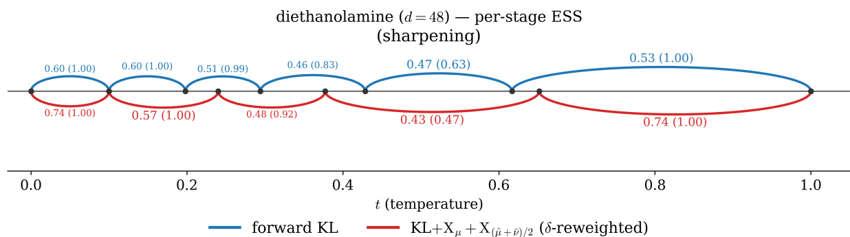
Figure 16: Diethanolamine per-stage ESS as annealing-ladder arcs (sharpening schedule): forward KL above the axis (blue), \text{KL} + X_\mu + X_{(\bar{\mu} + \bar{\nu})/2} , \delta -reweighted, below (red). Each arc is an accepted stage; the apex label is that stage's validation ESS, with the sharpening ESS in parentheses.
