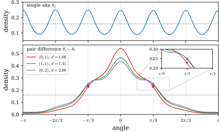
Figure 7: Angle densities from 2 \times 10^6 fresh samples advanced through the trained B = 2000 \text{KL} + X_\mu + X_{(\hat{\mu} + \bar{\nu})/2} stage sequence by map, reweighting, resampling, and MALA. The upper panel is the single-site marginal. The lower panel gives pair differences at offsets (0, 1), (1, 1), and (0, 2); dots and the inset resolve the one-clock-step angle \pi/3 . Dashed lines show the uniform density.
