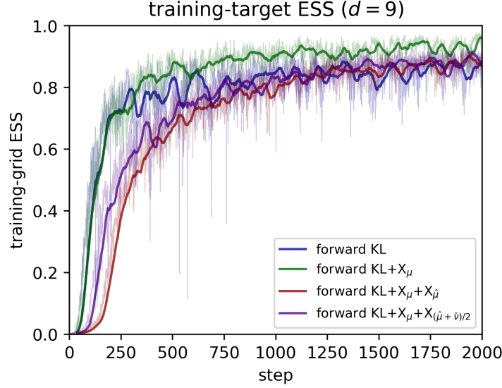
Figure 4: In-batch training-target ESS over 2000 steps on the Bayesian Fourier benchmark (28), four methods. Every method’s per-step ESS climbs above 0.85, so the training-time ESS itself does not reveal which methods have placed mass on more than one of the four posterior modes; the fresh-pool ESS and the coverage column in Table 3 are the actual discriminators.
