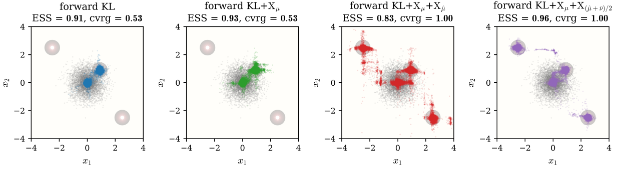
Figure 4: Sparse target. Columns show forward KL, \text{KL} + X_\mu , \text{KL} + X_\mu + X_{\hat{\mu}} , and \text{KL} + X_\mu + X_{(\hat{\mu} + \bar{\nu})/2} , with the learned pushforward overlaid on the target energy; panel titles report final ESS and coverage, and gray points show the source. The first two objectives cover the central pair but miss the two remote modes. The \hat{\mu} -only objective restores the remote modes with visible mass between components, whereas the equal mixture covers all four modes with less intermodal mass and higher ESS.
