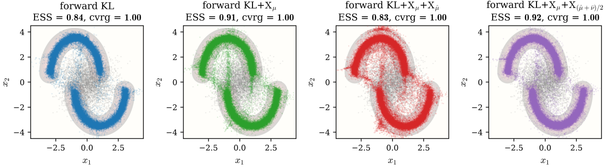
Figure 1: Two-Moon target. Columns, from left to right, are forward KL, \text{KL}+\text{X}_\mu , \text{KL}+\text{X}_\mu+\text{X}_{\hat{\mu}} , and \text{KL}+\text{X}_\mu+\text{X}_{(\hat{\mu}+\bar{\nu})/2} . Each panel overlays the pushforward samples on the target energy and reports final ESS and coverage. Gray points show the source.
