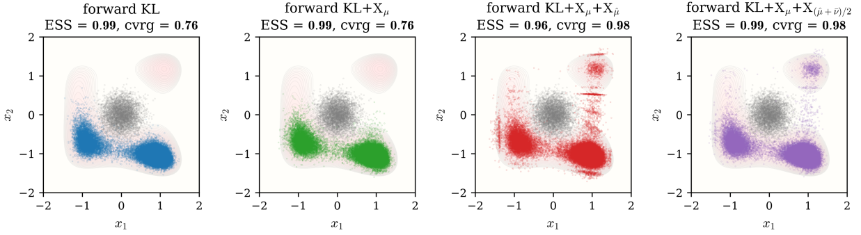
Figure 2: Three-Well target. From left to right, the panels show forward KL, \text{KL}+\text{X}_\mu , \text{KL}+\text{X}_\mu+\text{X}_{\hat{\mu}} , and \text{KL}+\text{X}_\mu+\text{X}_{(\hat{\mu}+\bar{\nu})/2} . Each panel overlays the pushforward samples on the target energy and reports final ESS and coverage; gray points show the source.
