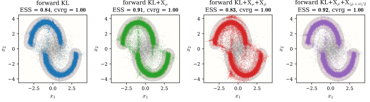
Figure 1: Two-Moon target. Columns, from left to right, are forward KL, KL+ X_\mu , KL+ X_\mu + X_{\hat{\mu}} , and KL+ X_\mu + X_{(\hat{\mu}+\bar{\nu})/2} . Each panel overlays the pushforward samples on the target energy and reports final ESS and coverage. Gray points show the source.
