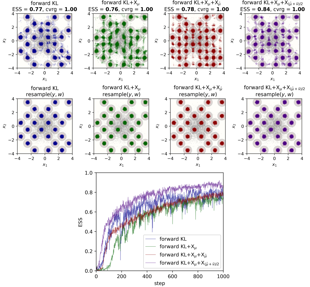
Figure 3: Chessboard target. Row 1: pushforward y = G^{-1}(x) . Row 2: resample( y, w ) with Langevin rejuvenation. Columns as in Figure 1. Row 3: ESS trajectory across training steps – bare forward KL and KL+ X_{\mu} fluctuate strongly throughout training, while the wide-coverage X_{\hat{\mu}} and mixture variants settle into markedly steadier curves, with the mixture both the highest and the tightest.
