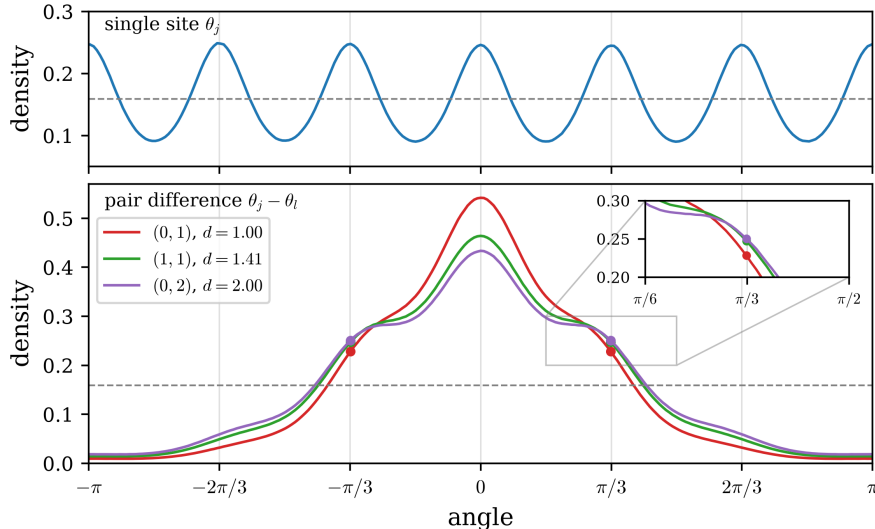
Figure 7: Angle densities from 2 \times 10^6 fresh samples advanced through the trained B = 2000 \text{KL} + X_\mu + X_{(\hat{\mu} + \bar{v})/2} ladder by map, reweighting, resampling, and MALA. The upper panel is the single-site marginal. The lower panel gives pair differences at offsets (0,1) , (1,1) , and (0,2) ; dots and the inset resolve the one-clock-step angle \pi/3 . Dashed lines show the uniform density.
