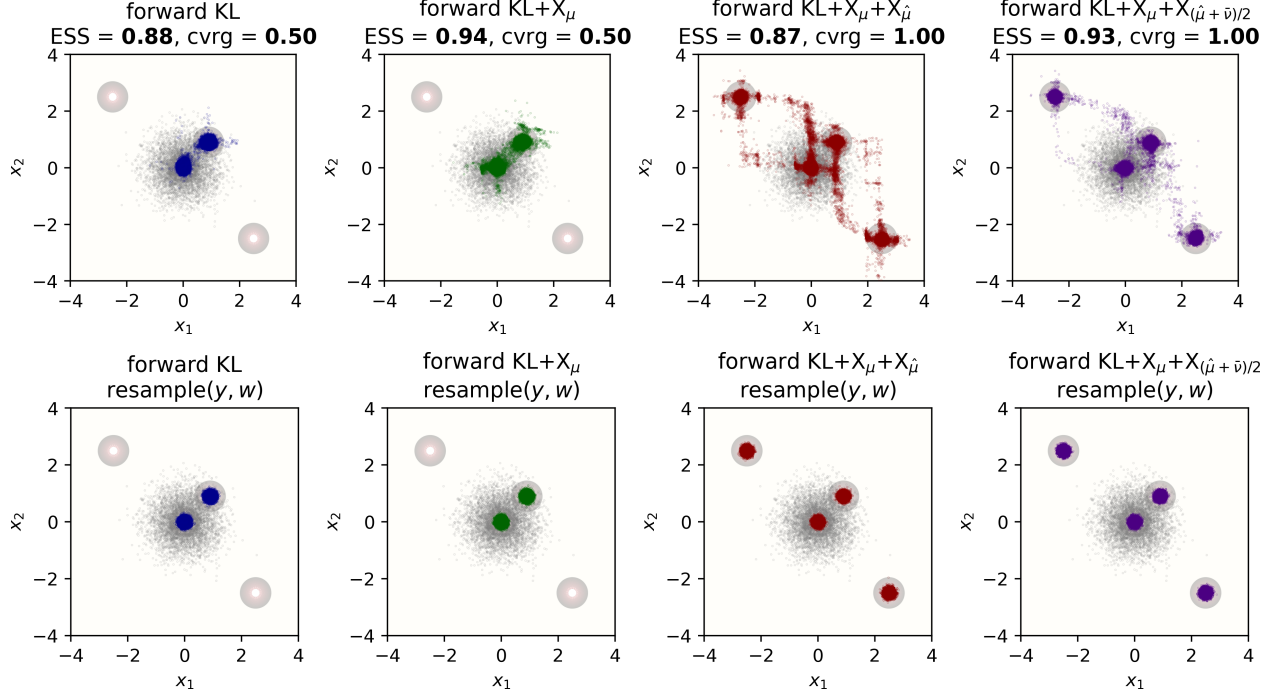
Figure 4: Sparse target. Row 1: pushforward y = G^{-1}(x) . Row 2: \text{resample}(y, w) with Langevin rejuvenation. Columns as in Figure 1. Forward KL and \text{KL}+X_\mu collapse onto the two central modes and miss both isolated corners at high, stable ESS (a fake-ESS instance); X_{\hat{\mu}} recovers all four modes but leaves artificial bridges of mass between them, while the mixture recovers them cleanly.
